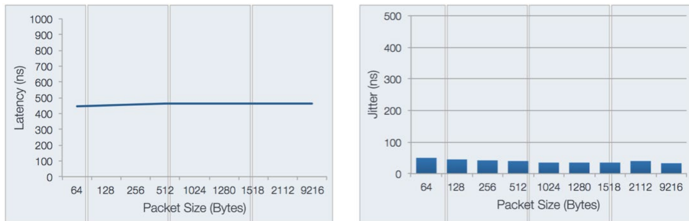
Figure 3: Arista 7060X &amp; 7260X forwarding latency and jitter
