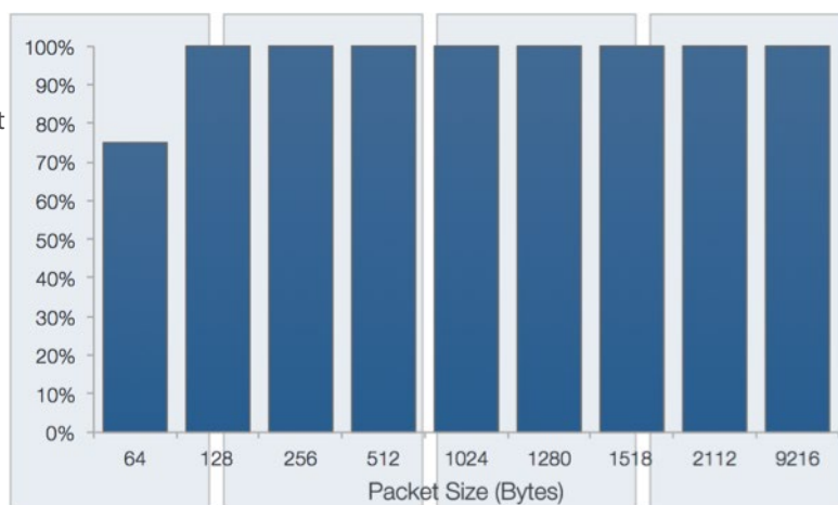
Figure 2: Arista 7060X &amp; 7260X throughput
