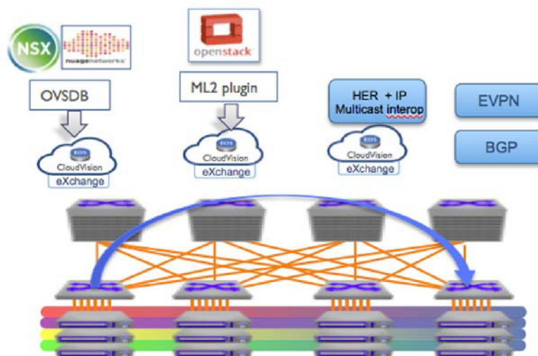
Figure 23-1: Different VXLAN Control Planes
