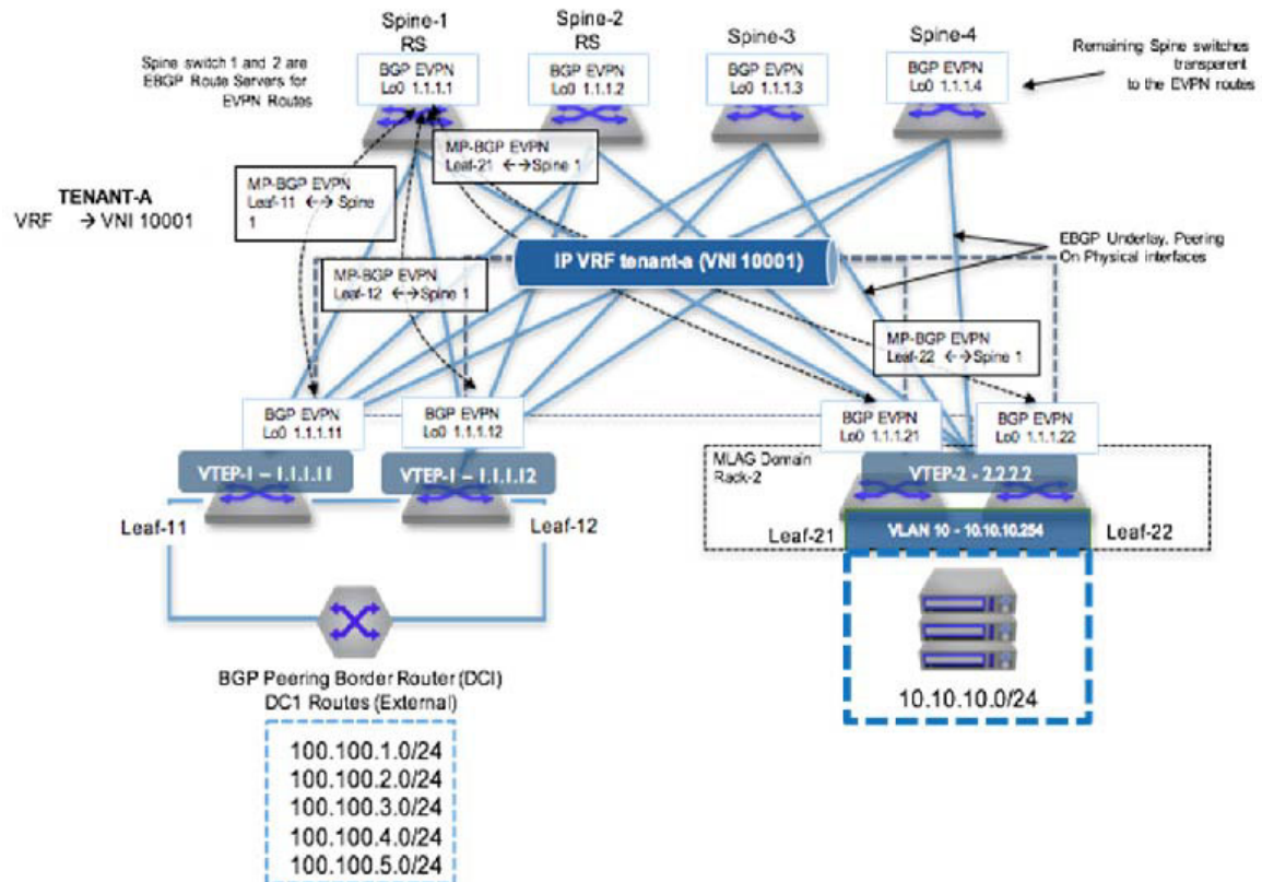
Figure 23-43: Layer 3 EVPN Configuration
