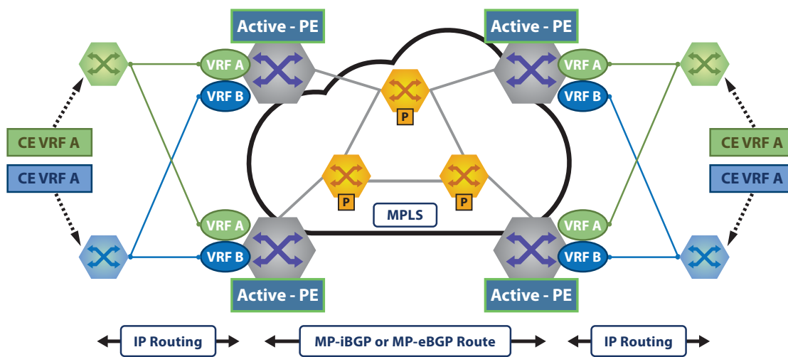
Figure 23-27: MPLS Layer 3 VPN Topology
