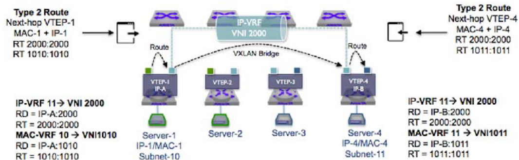
Figure 23-19: EVPN Symmetric IRB
