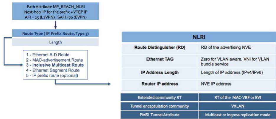
Figure 23-15: EVPN Type-3 IMET Route Format
