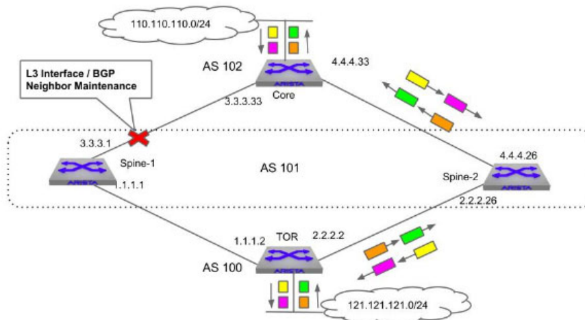
Figure 10-2: Traffic flow pattern between TOR and Core – After unit on Spine-1 is put into Maintenance
