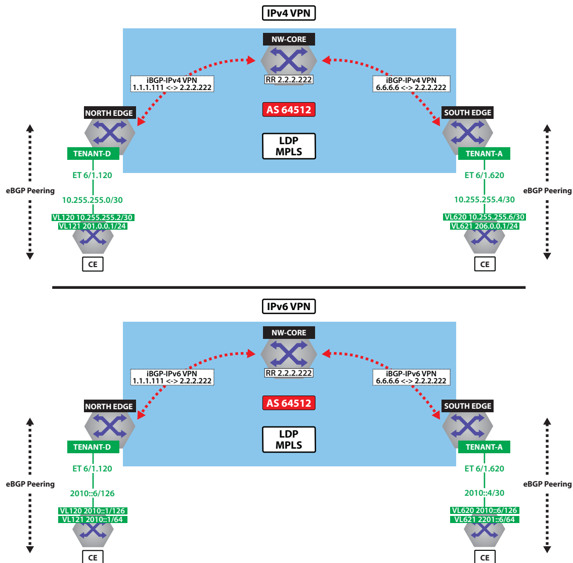
Figure 23-61: IPv4 VPN and IPv6 VPN Over LDP MPLS
