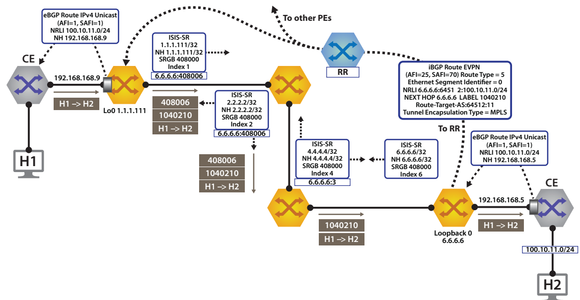
Figure 23-49: Control Plane &amp; Forwarding Tenant-a Over ISIS-SR
