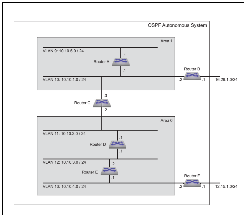
Figure 31-5: OSPFv2 Example 3
