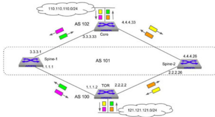
Figure 10-1: Traffic flow pattern between TOR and Core – Before Maintenance
