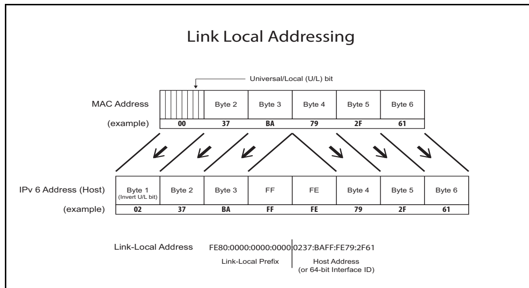
Figure 29-1: Link Local Address Derivation
