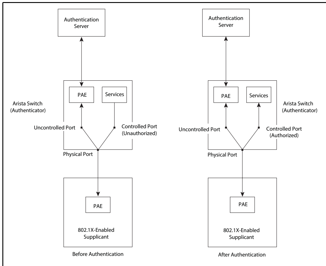
Figure 14-3: Ports before and after client authentication
