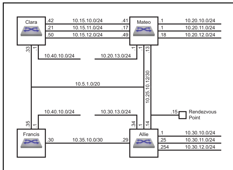
Figure 40-1: Multicast Example
