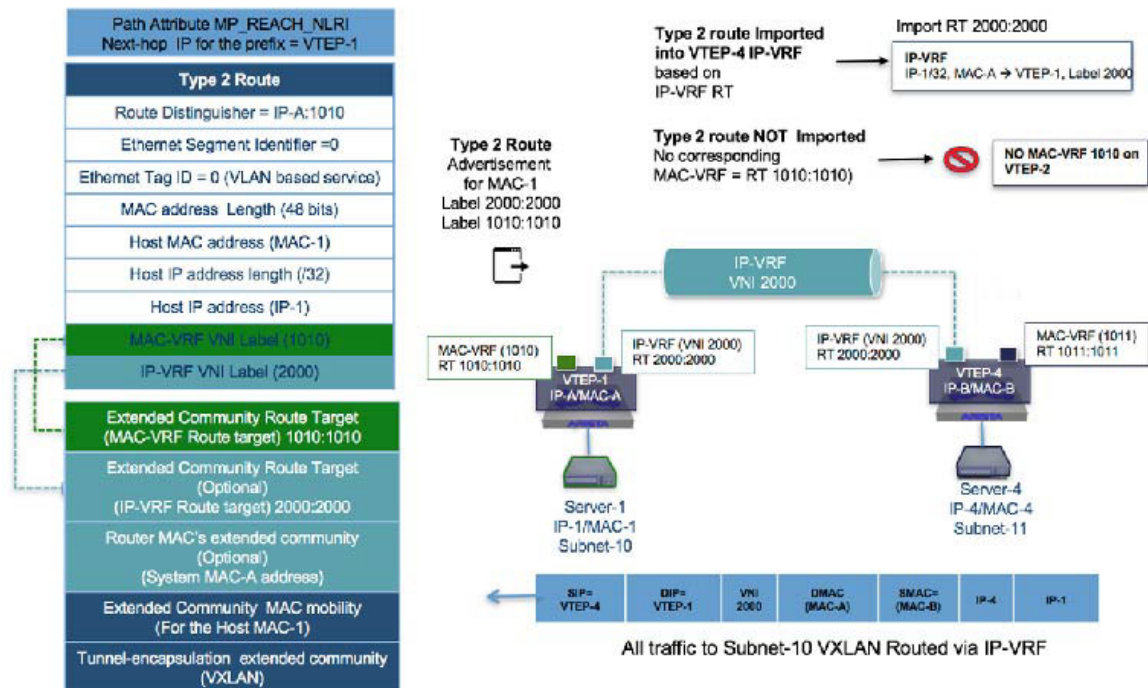
Figure 23-21: EVPN Type 2 Route in Symmetric IRB - MAC-VRF Only Exists on Sending VTEP
