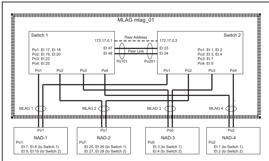
Figure 13-3: MLAG Implementation Example
