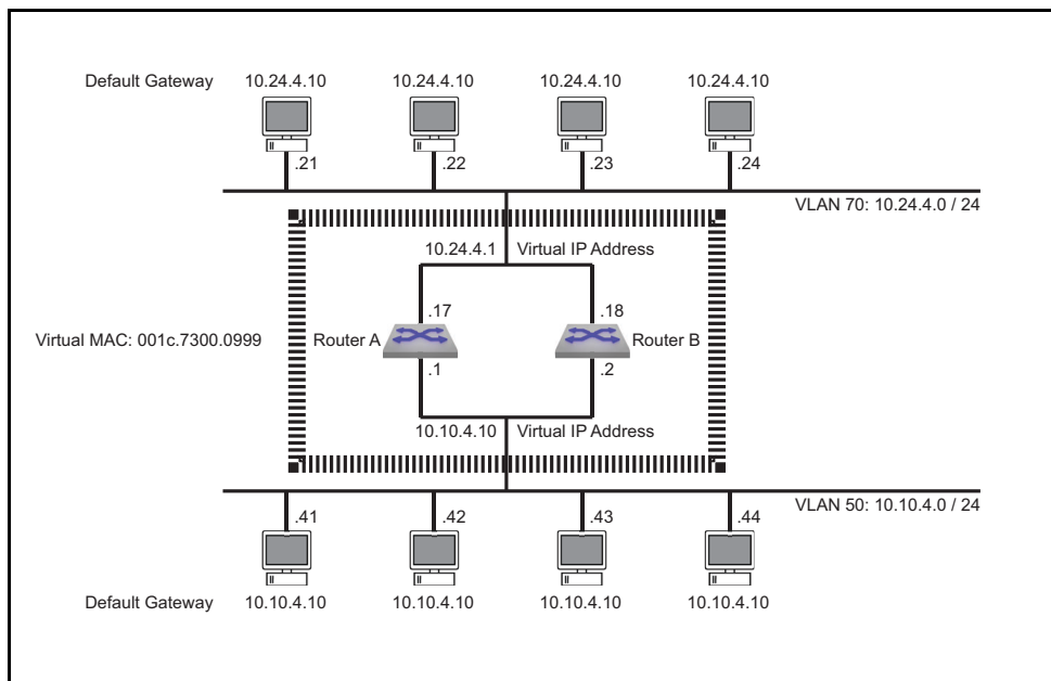
Figure 25-5: VARP Example Network Diagram
