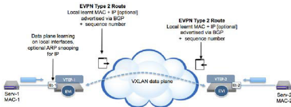
Figure 23-11: EVPN Type 2 Route Announcement
