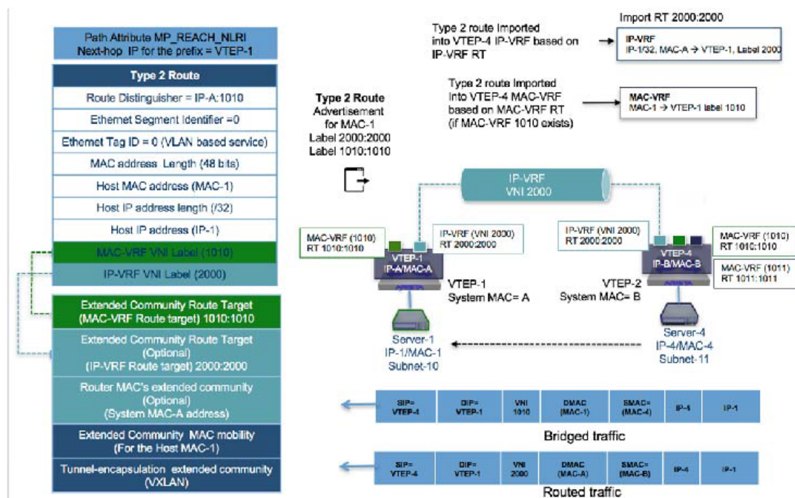
Figure 23-20: EVPN Type 2 Route in Symmetric IRB - MAC-VRF on Both VTEPs
