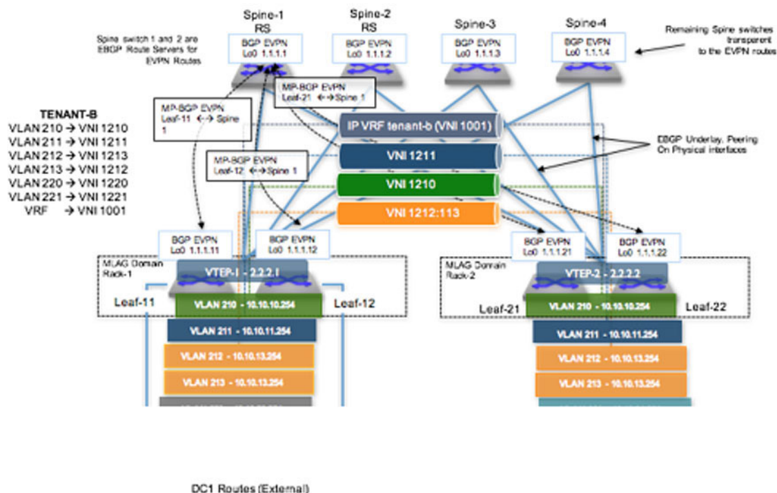
Figure 23-45: Tenant-B: Asymmetric IRB
