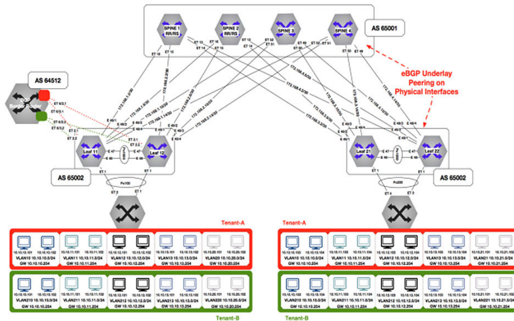
Figure 23-46: Physical Underlay Topology
