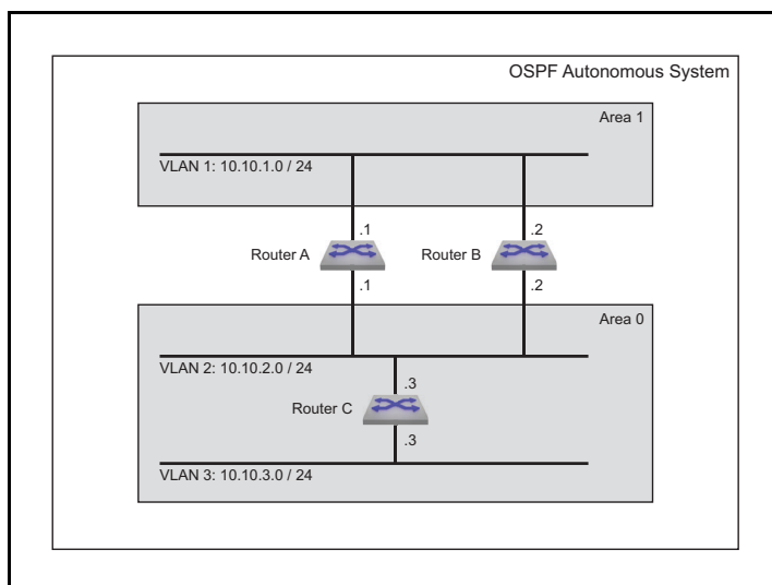
Figure 31-3: OSPFv2 Example 1
