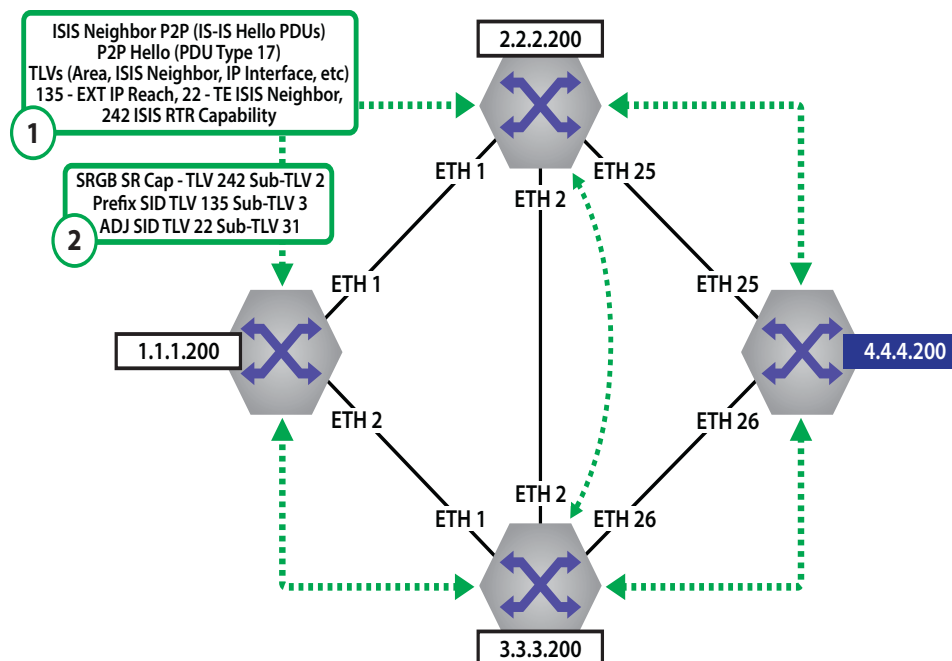
Figure 23-35: ISIS Neighbor Adj and TLVs
