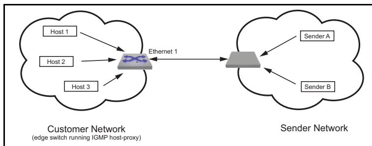
Figure 39-1: IP IGMP Host Proxy Implementation
