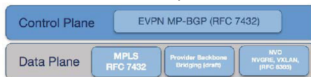
Figure 23-2: VXLAN Control Plane and Data-plane Definitions
