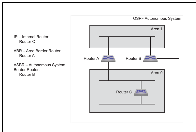
Figure 31-1: OSPFv2 Router Types
