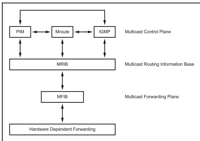
Figure 38-1: Multicast Architecture
