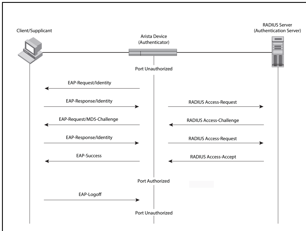
Figure 14-4: Message exchange during authentication
