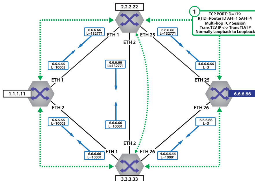
Figure 23-36: BGP-LU Label Distribution
