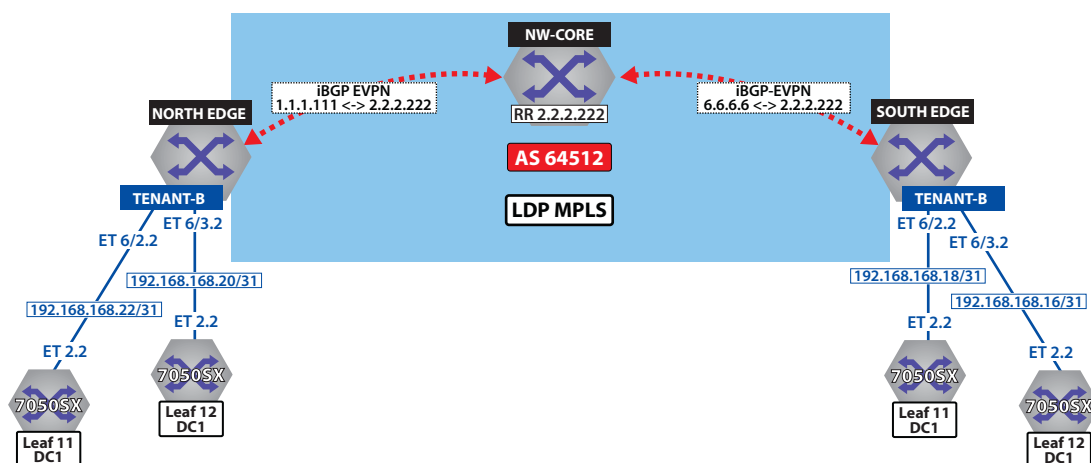
Figure 23-51: Control Plane Tenant-B over LDP
