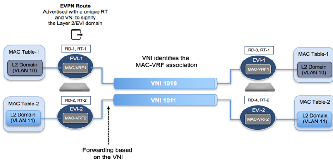
Figure 23-5: VLAN Based Service Interface
