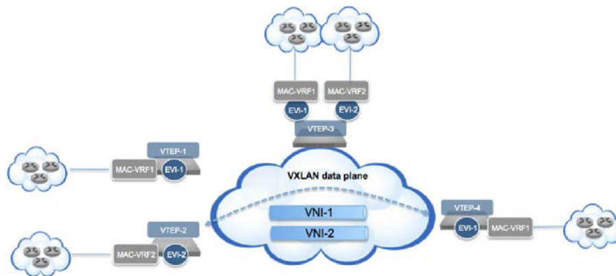
Figure 23-3: EVPN Terminology for a VXLAN Data Plane
