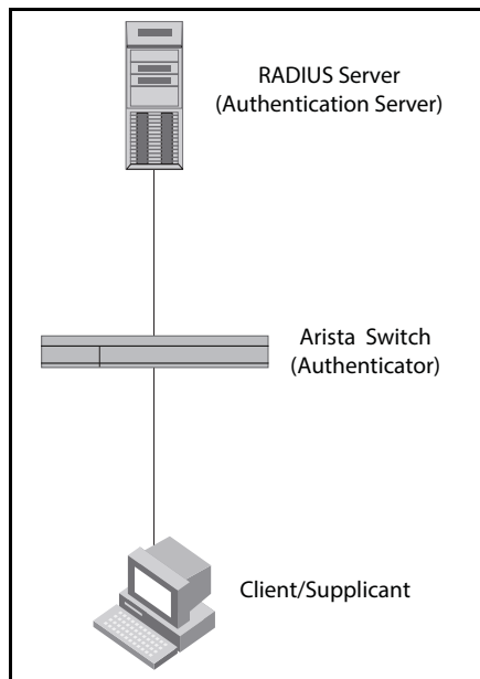
Figure 14-1: Authenticator, Supplicant, and Authentication Server in an 802.1X configuration
