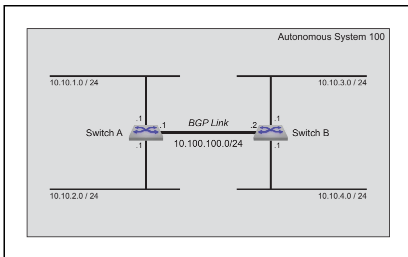
Figure 33-2: BGP Example 1
