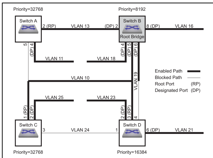
Figure 26-1: Spanning Tree Network Example
