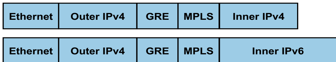
Figure 36-1: Header Format of Packets
