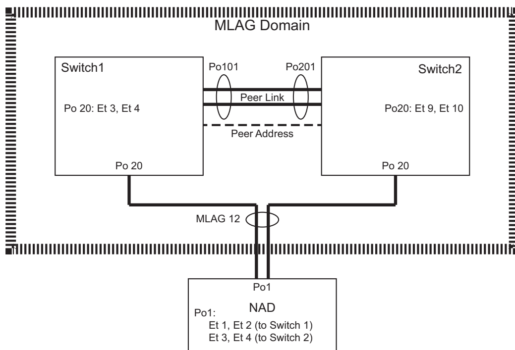
Figure 13-2: MLAG Interface Configuration
