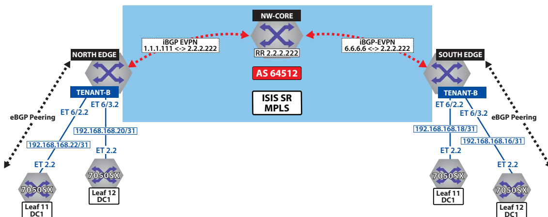
Figure 23-48: Control Plane Tenant-B over ISIS-SR
