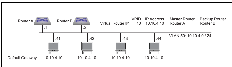
Figure 25-2: VRRP Example 1 Network Diagram
