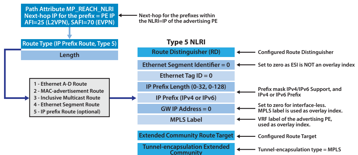
Figure 23-9: EVPN Route Type-5, for Advertisement of IP-Prefixes over MPLS
