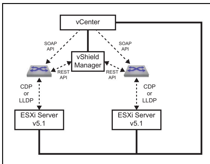
Figure 45-2: VM Tracer Topology – Monitoring VXLAN Based Configurations
