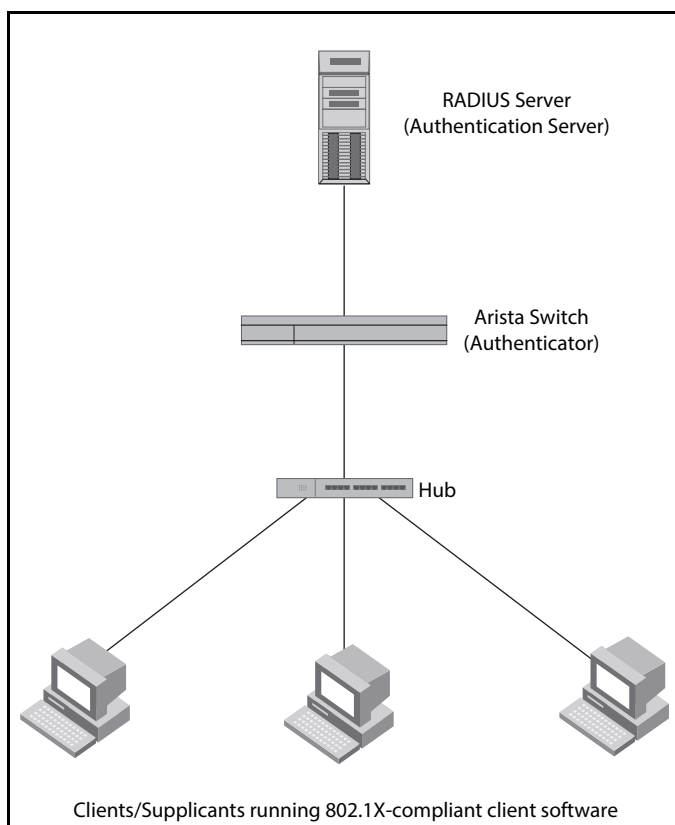
Figure 14-5: Multiple clients connected to a 802.1X-enabled port
