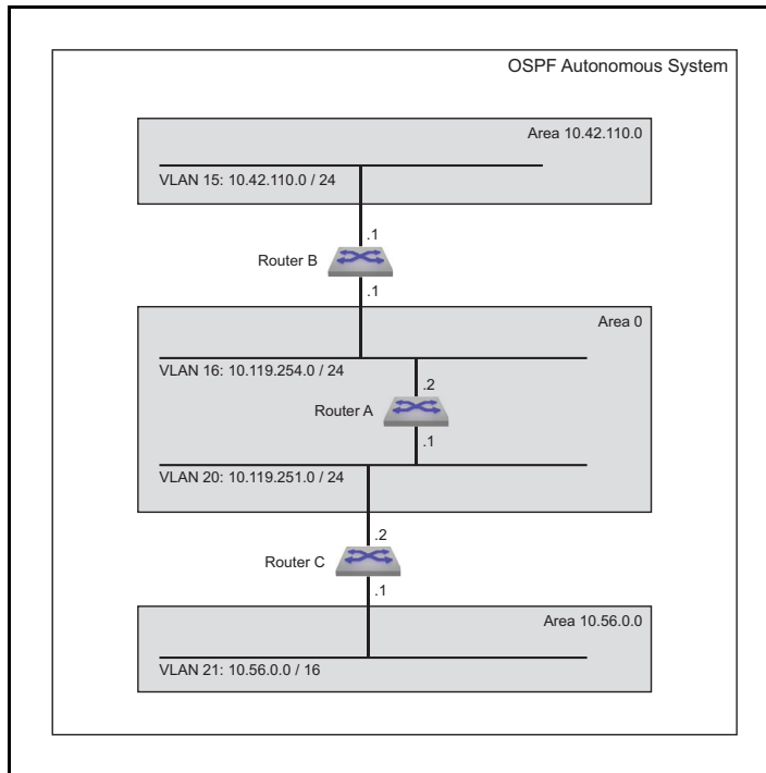
Figure 31-4: OSPFv2 Example 2
