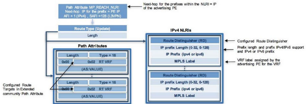
Figure 23-24: IPv4 and IPv6 VPN Update Route Detail
