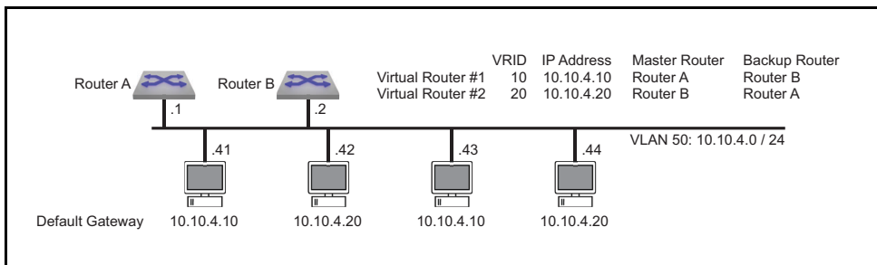
Figure 25-3: VRRP Example 2 Network Diagram
