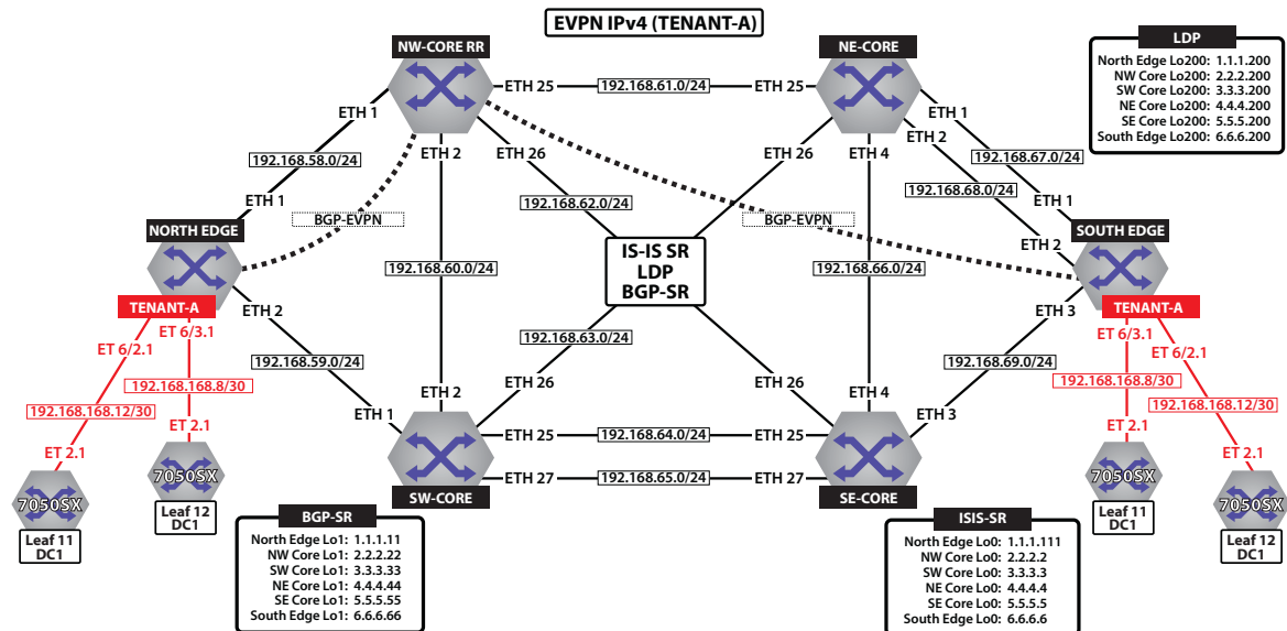
Figure 23-29: Tenant-A DCI
