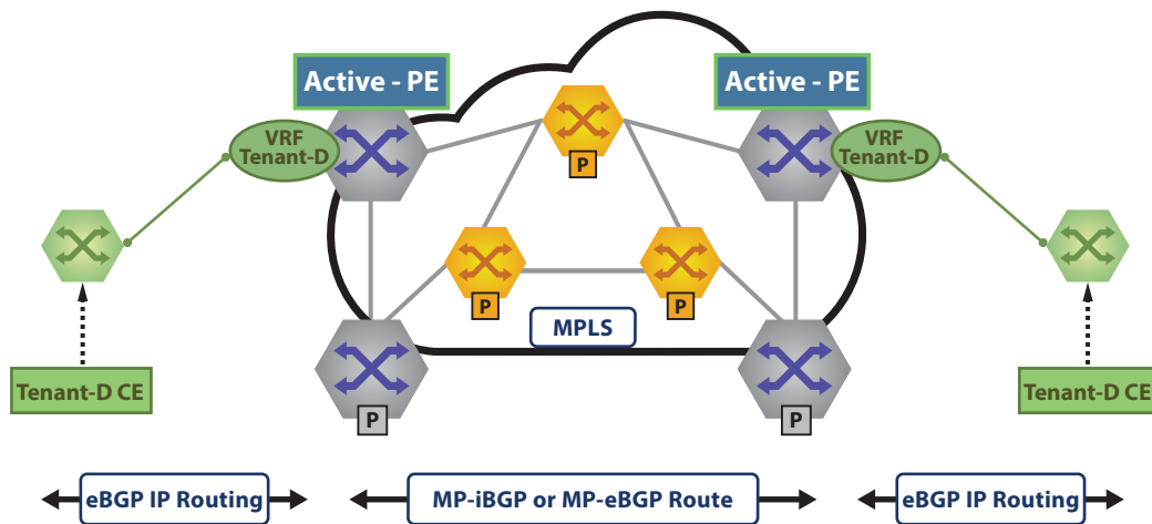
Figure 23-31: IPv4 & IPv6 VPN Sample Topology
