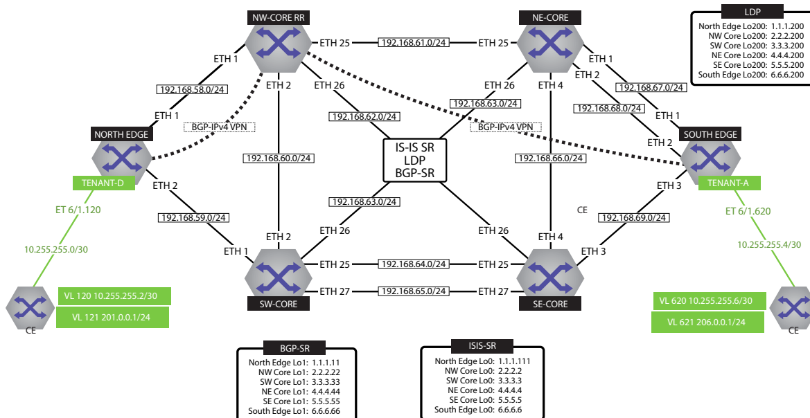
Figure 23-56: IPv4 VPN Physical Topology
