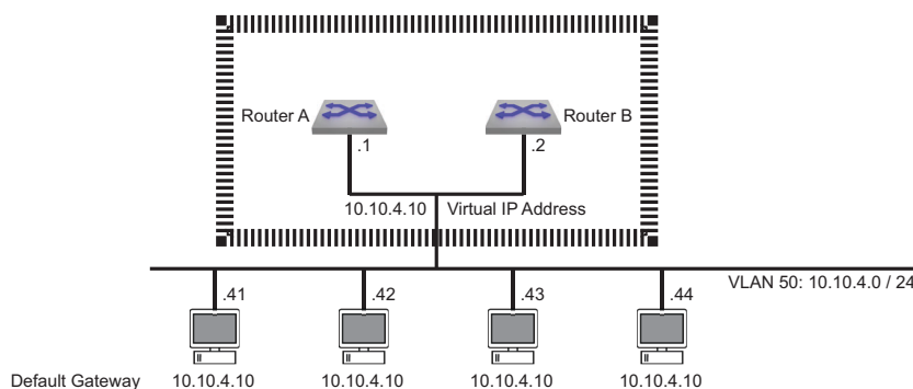
Figure 25-1: VARP Configuration
