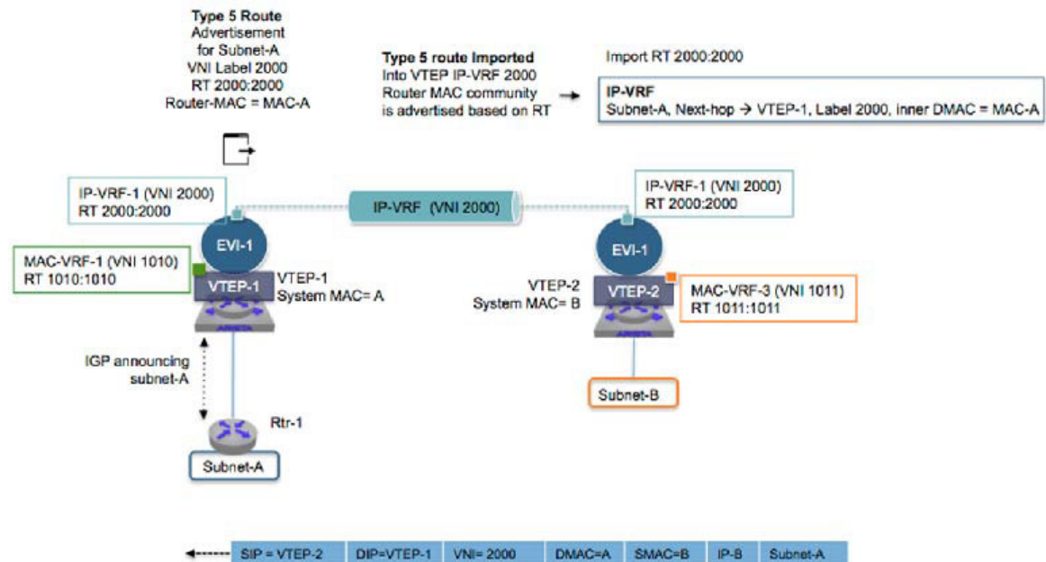
Figure 23-39: EVPN Route Type-5, Interface-less Update
