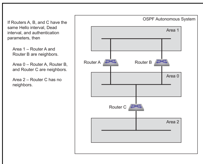
Figure 31-2: OSPFv2 Neighbors
