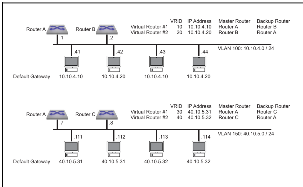
Figure 25-4: VRRP Example 3 Network Diagram
