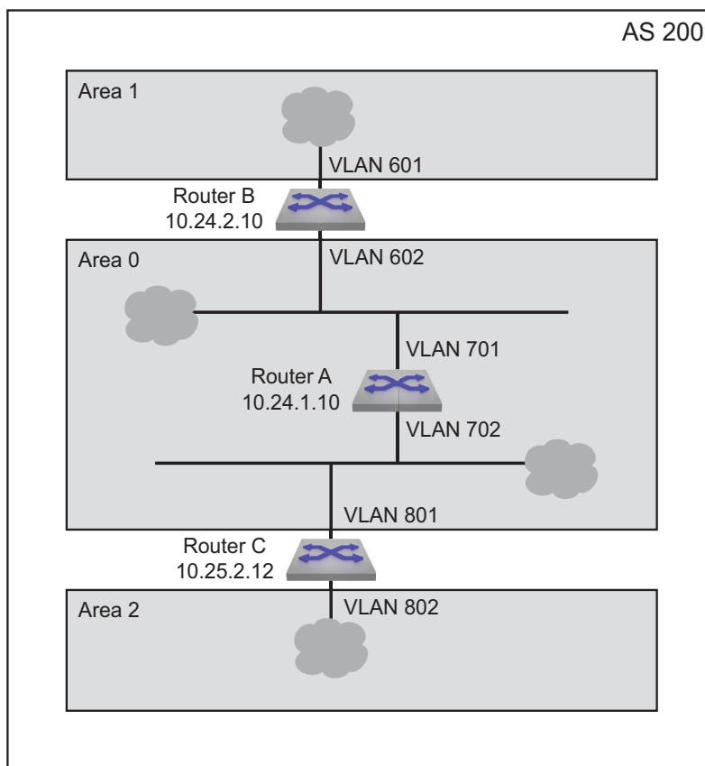
Figure 32-4: OSPFv3 Example 2
