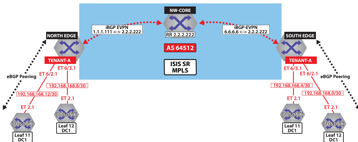
Figure 23-47: Control Plane Tenant-A Over ISIS-SR
