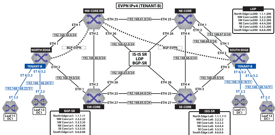
Figure 23-30: Tenant-B DCI
