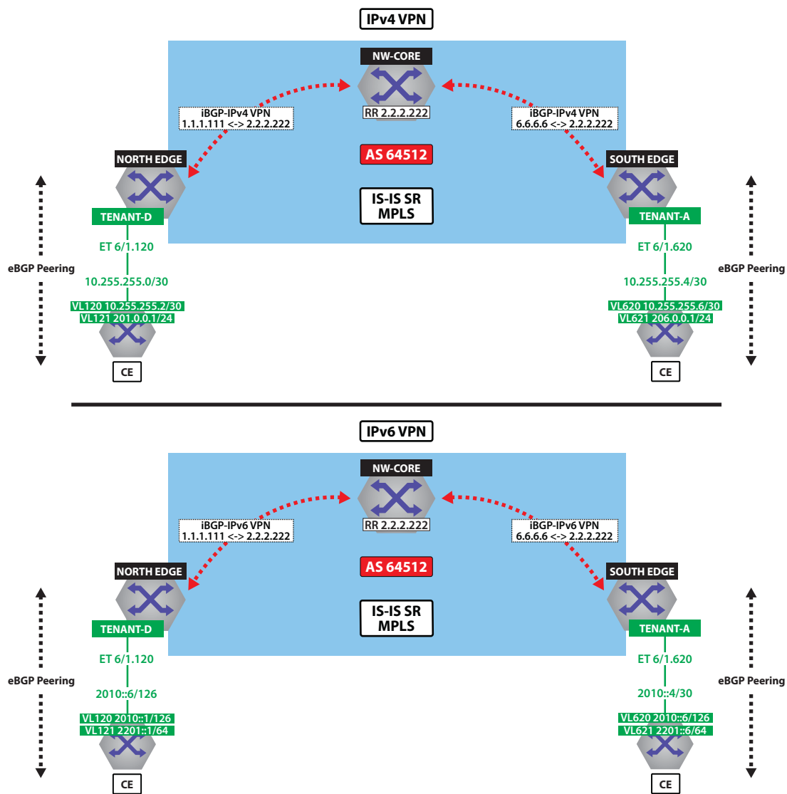
Figure 23-58: IPv4 VPN and IPv6 VPN Over ISIS-SR MPLS
