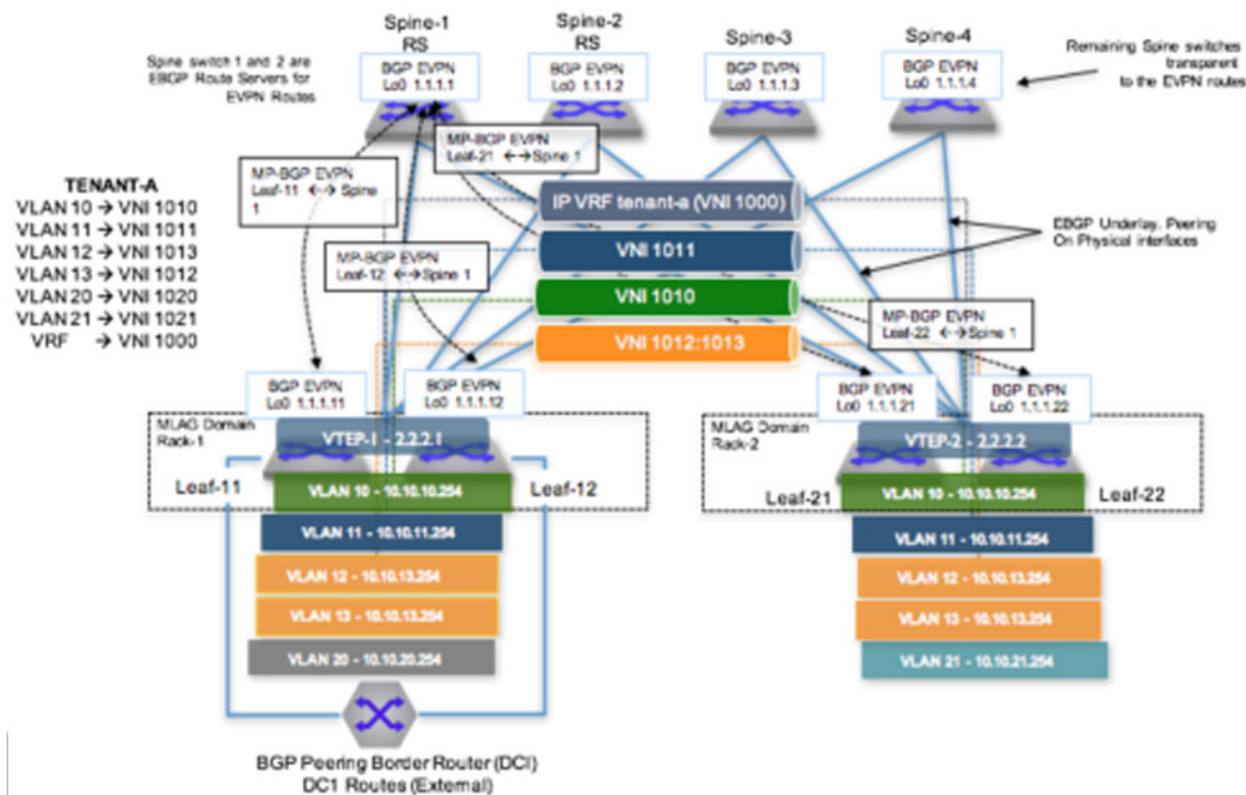
Figure 23-44: Tenant-A: Symmetric IRB
