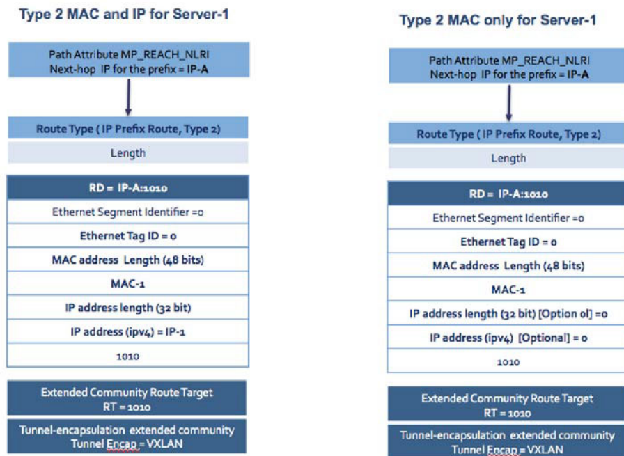
Figure 23-17: EVPN Comparison of MAC & MAC+IP Type 2 Route in Asymmetric IRB
