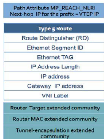
Figure 23-38: EVPN Route Type-5, for Advertisement of IP Prefixes
