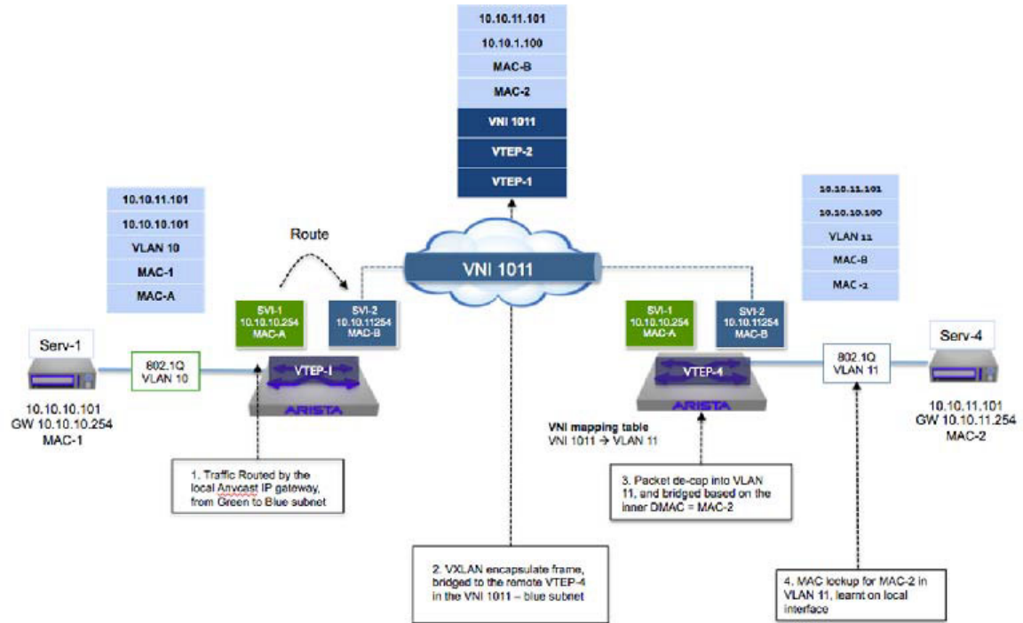
Figure 23-18: EVPN Asymmetric IRB VxLAN Data-plane Forwarding Detail
