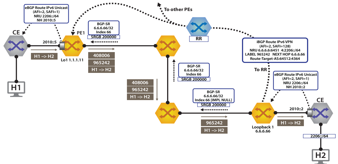
Figure 23-66: IPv6 VPN Forwarding Over BGP-SR MPLS
