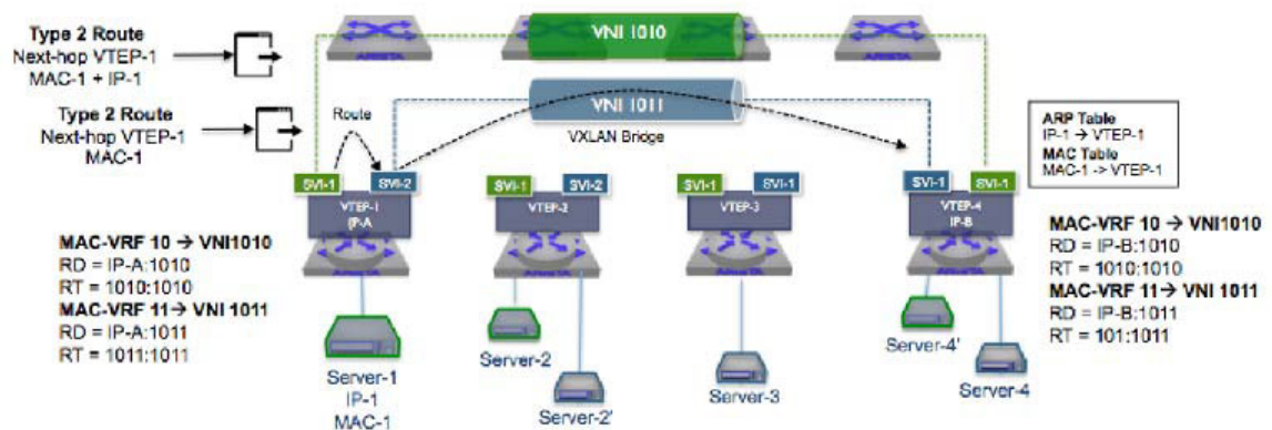
Figure 23-16: EVPN Asymmetric IRB
