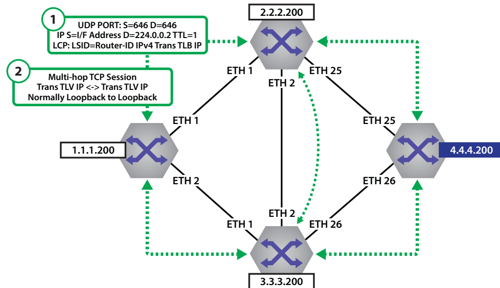
Figure 23-34: LDP Peering Establishment
