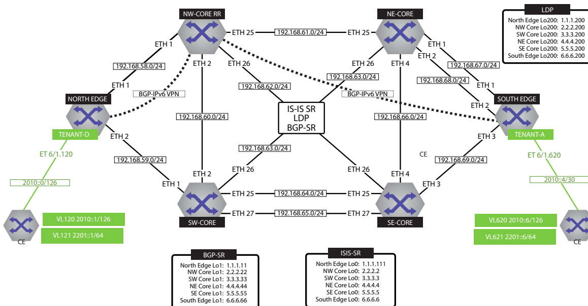
Figure 23-57: IPv6 VPN Physical Topology
