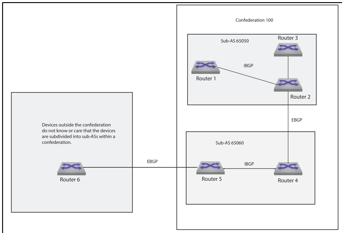
Figure 33-1: BGP Confederation Example
