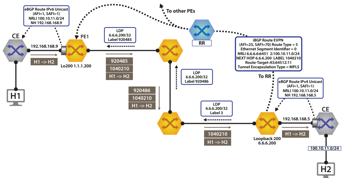
Figure 23-52: Control Plane &amp; Forwarding Tenant-a Over LDP
