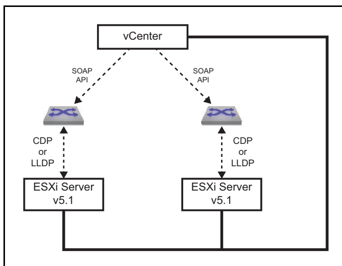
Figure 45-1: VM Tracer Topology – Monitoring VLAN Based Configurations
