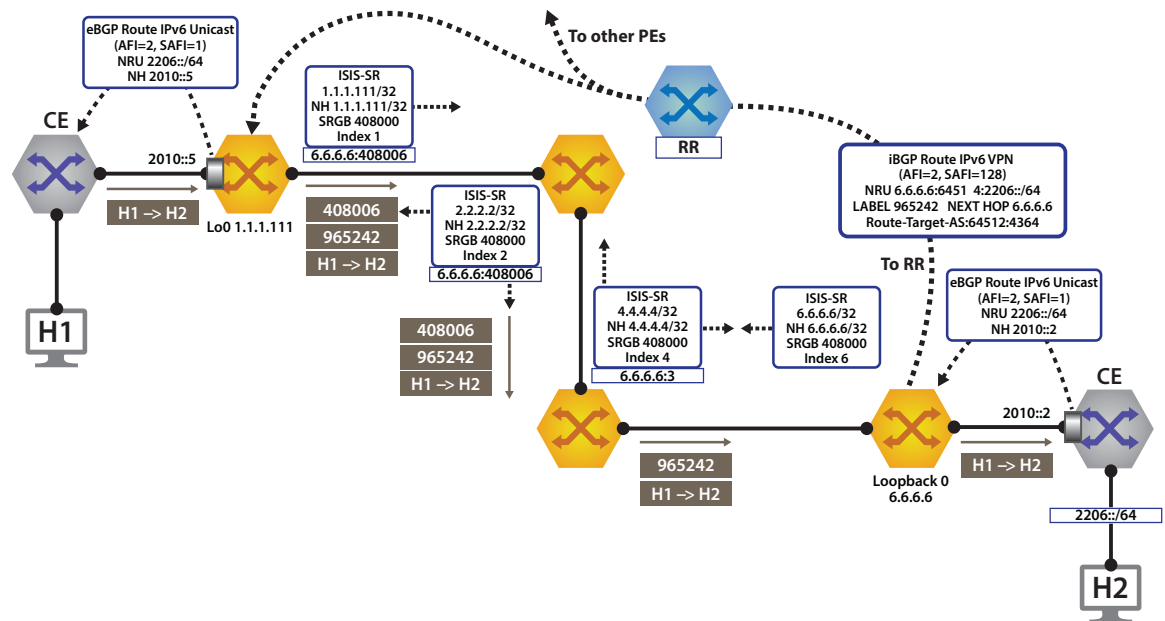
Figure 23-60: IPv6 VPN Forwarding Over ISIS-SR MPLS
