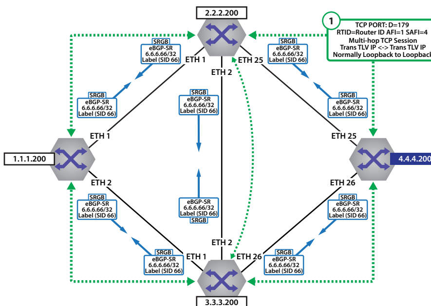
Figure 23-37: BGP-SR Index and SRGB Distribution
