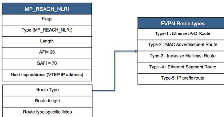
Figure 23-4: EVPN NLRI Route Format
