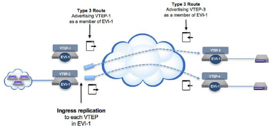
Figure 23-14: EVPN type-3 IMET Route Behavior for Ingress Replication
