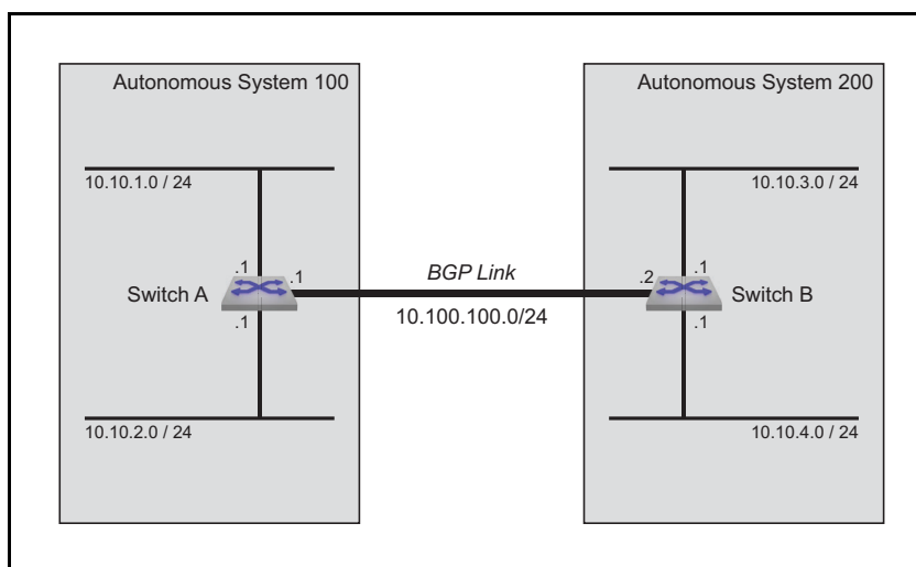
Figure 33-3: BGP Example 2
