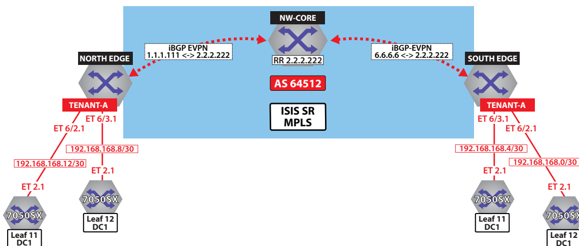
Figure 23-50: Control Plane Tenant-A Over LDP
