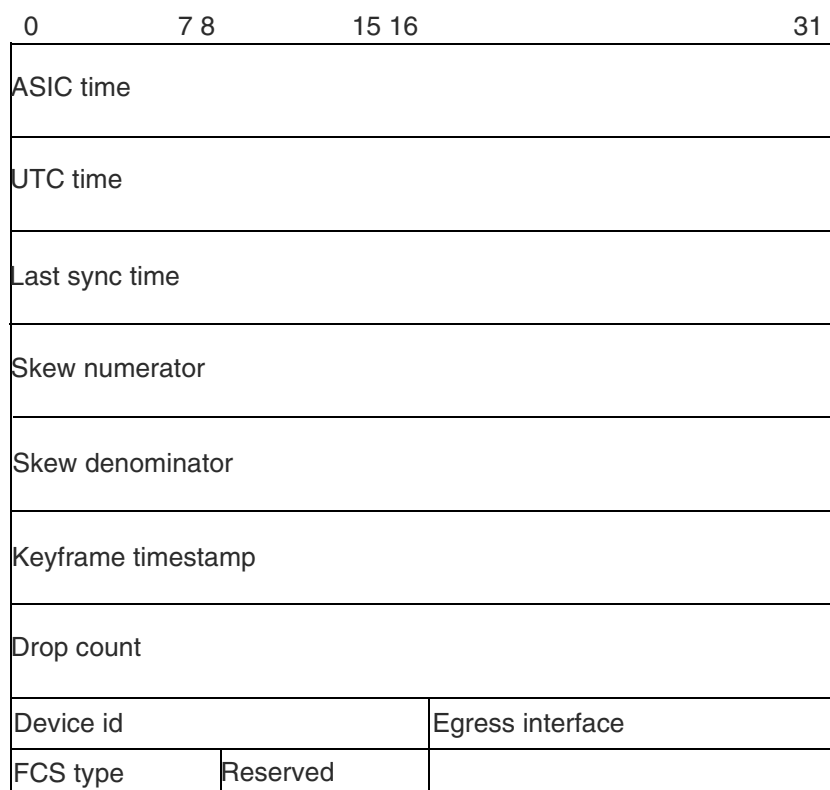
Figure 20-1: Key frame payload
