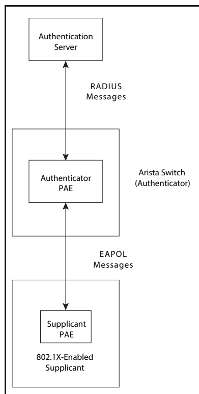
Figure 14-2: Authenticator PAE and Supplicant PAE
