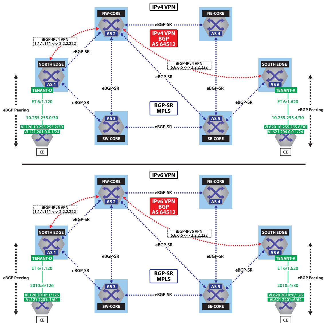
Figure 23-64: IPv4 VPN and IPv6 VPN Over BGP-SR MPLS
