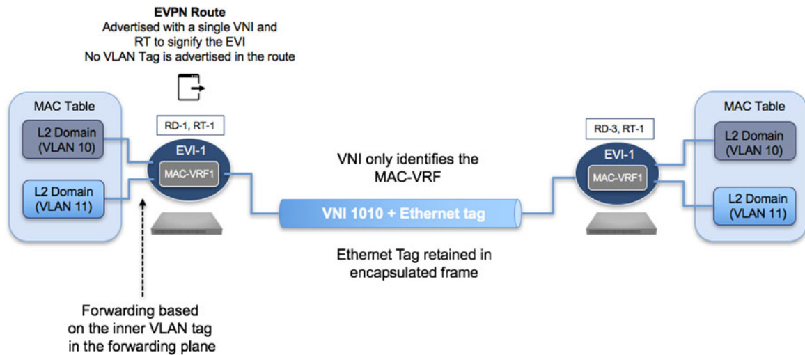
Figure 23-6: VLAN Bundle Service Interface
