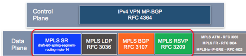
Figure 23-22: MPLS data-plane
