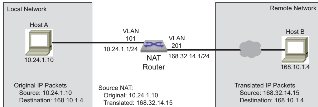
Figure 28-5: Destination NAT Example
