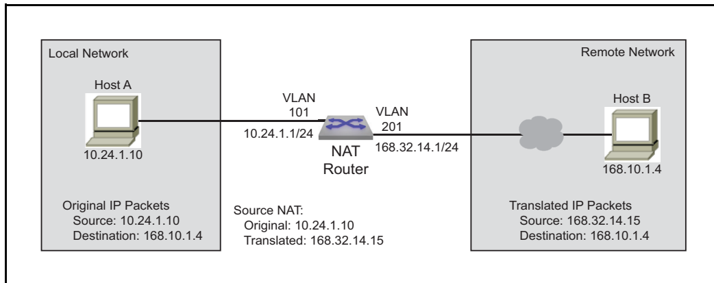
Figure 28-4: Source NAT Example
