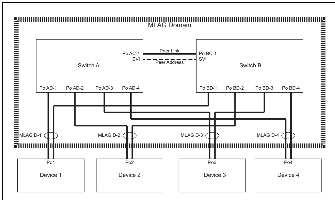
Figure 13-1: MLAG Domain Topology
