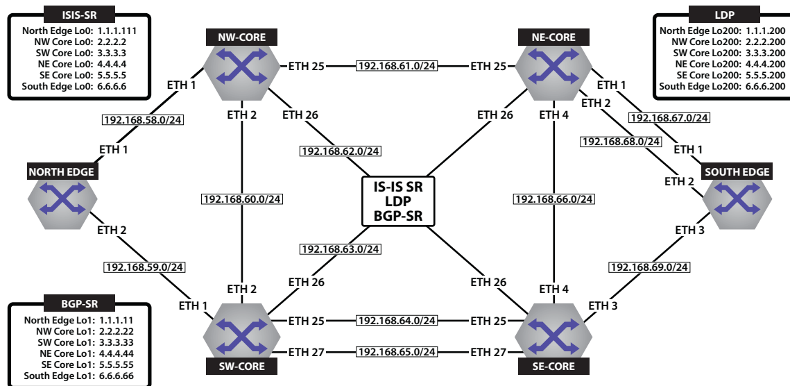
Figure 23-28: Physical Topology For ISIS-SR, LDP and BGP-SR Transport
