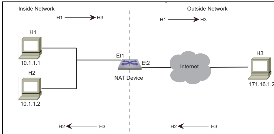
Figure 28-6: Dynamic NAT Scenario
