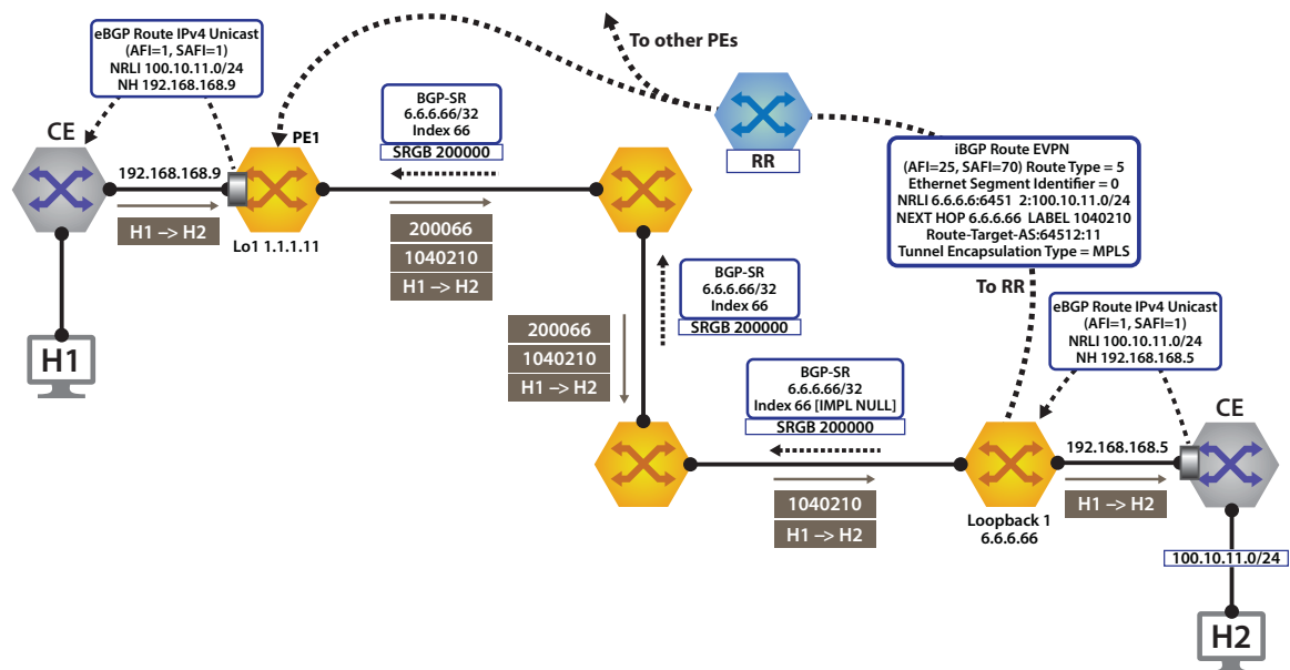
Figure 23-55: Control Plane &amp; Forwarding Tenant-a Over BGP-SR
