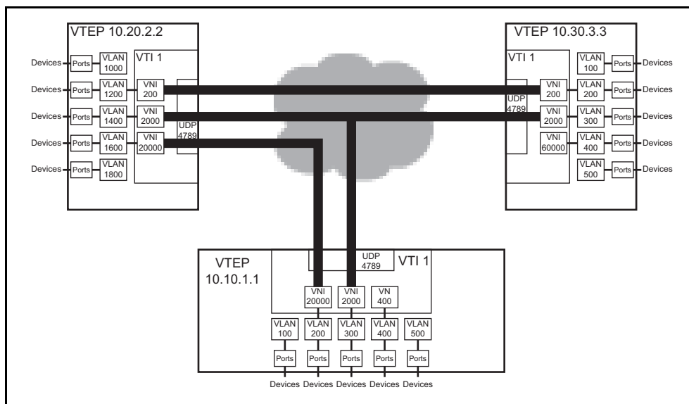
Figure 22-2: VXLAN Implementation
