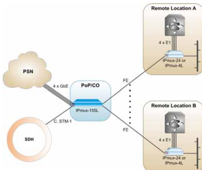
Figure 2. Aggregating Pseudowire Traffic from Remote Locations
