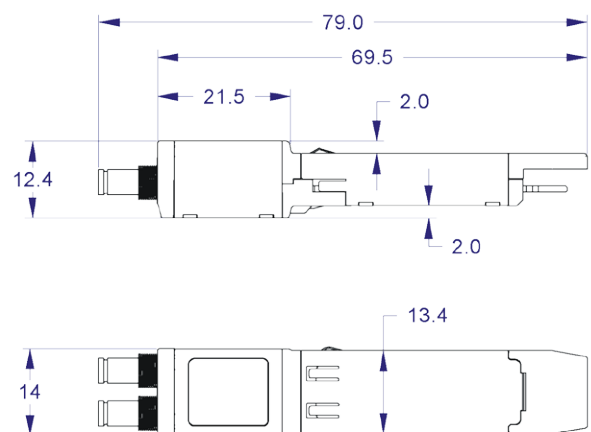
Figure 2. Physical Dimensions
